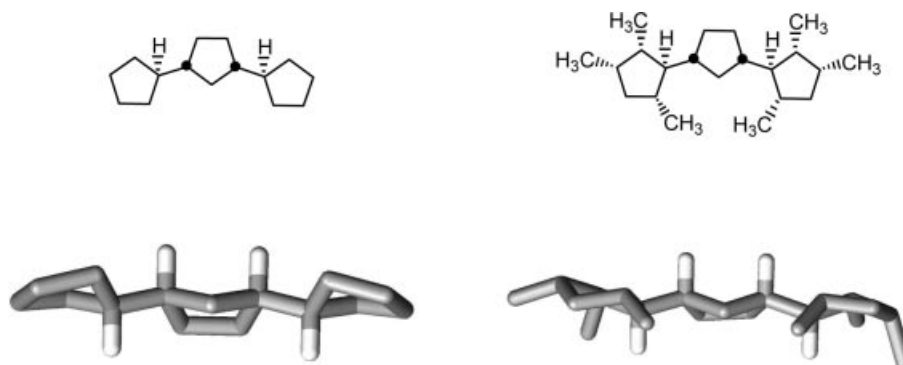
Figure 3. Starting conformations for ter -cyclopentane ( 6 , left) and hexamethyl ter -cyclopentane ( 7 , right) dihedral angle drives. Only protons flanking the critical torsion angles are shown.
