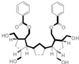
Figure 7. Torsional bonds varied (black lines) and ring closures (dotted lines) in restrained and unrestrained conformational analysis of 5 .
