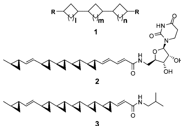
Figure 1. Examples of stereoregular oligocycloalkanes.
