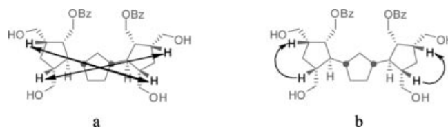
Figure 6. Hypothetical alternative NOE assignments for the 5,5''–3,3'' crosspeak.
