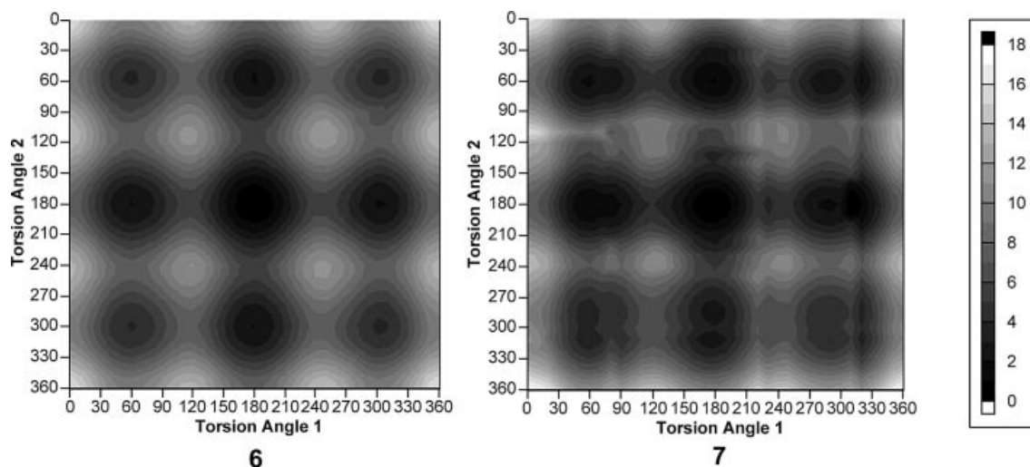
Figure 4. Dihedral angle drive for 6 and 7 . Legend indicates relative energy in kcal/mol.
