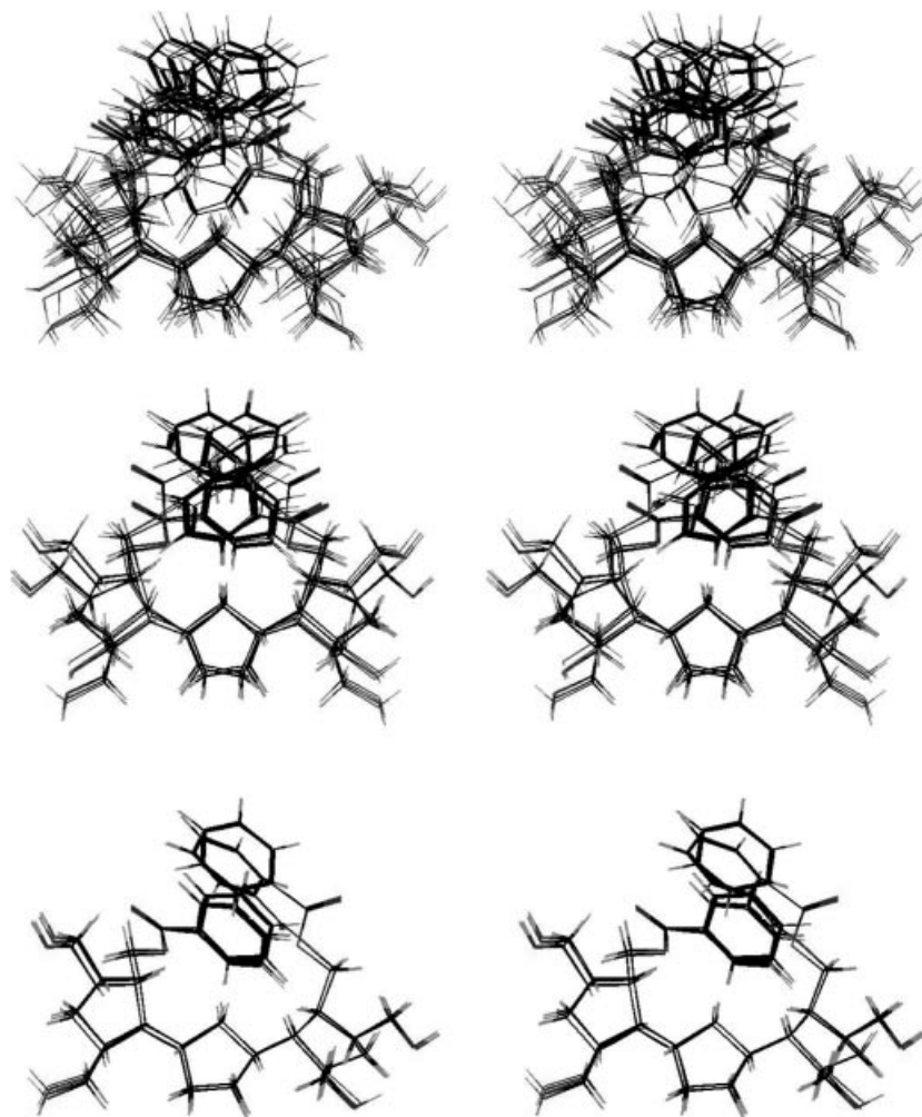
Figure 8. Wall-eyed stereoview of the overlay of the first 10 lowest energy output structures from conformation searches (MCMM, MMFFs, GB/SA H 2 O) for 5 in the absence of NMR-derived restraints (top, lowest 0.4 kcal/mol of output structures), in the presence of only NMR-derived distance restraints (middle, lowest 1.4 kcal/mol of output structures), and in the presences of both NMR-derived distance and torsional restraints (bottom, lowest 3.0 kcal/mol of output structures). This figure was generated with Maestro. [14]
