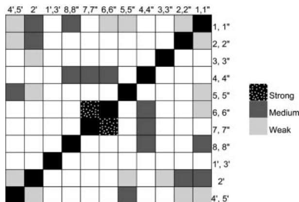
Figure 5. Distance restraints derived from the NOESY spectrum of 5 in CD 3 OD.
