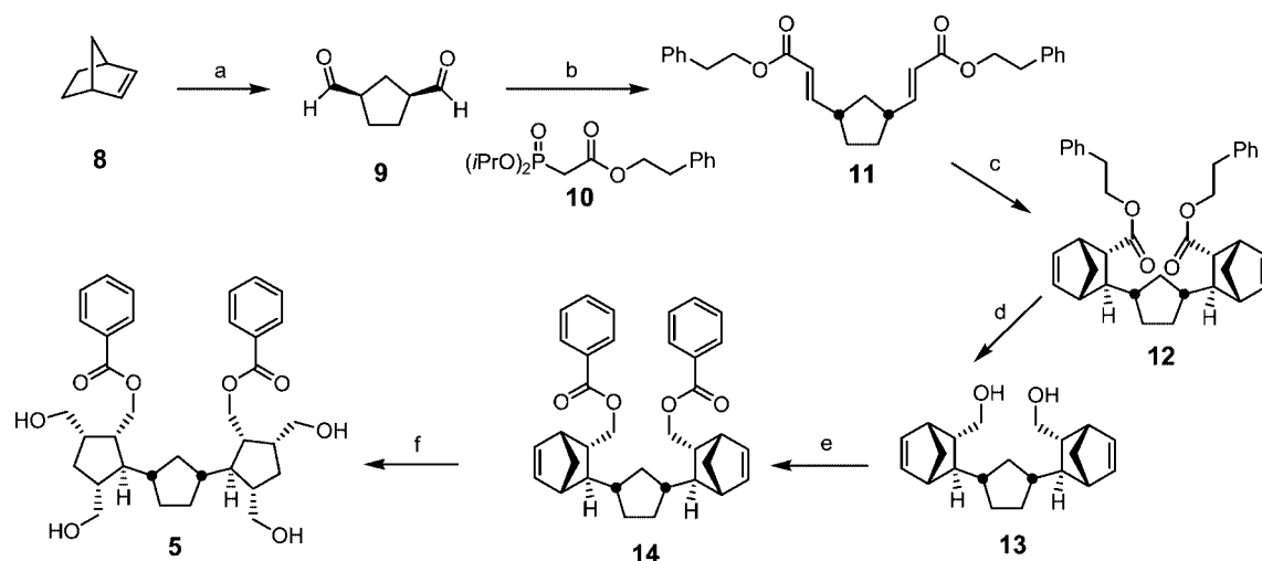
Scheme 1. (a) \text{KMnO}_4 on \text{CuSO}_4 , \text{CH}_2\text{Cl}_2 , room temp., 12 h; (b) \text{KO}^t\text{Bu} , THF, 0 °C to room temp. 2 h, then –78 °C, 10 , 10 h (61% over 2 steps); (c) (\text{CH}_3)_3\text{Al} (0.05 equiv.), \text{AlCl}_3 (0.5 equiv.), cyclopentadiene (10 equiv.), \text{CH}_2\text{Cl}_2 , 4 °C, 18 h (15%); (d) \text{LiAlH}_4 (6 equiv.), THF, room temp., 24 h (51%); (e) benzoyl chloride (3.6 equiv.), \text{Et}_3\text{N} (4 equiv.), \text{CH}_2\text{Cl}_2 , room temp., 3 h (35%); (f) \text{O}_3 , \text{CH}_2\text{Cl}_2/\text{CH}_3\text{OH} (1:1), –78 °C, 15 min., then \text{NaBH}_4 (20 equiv.), 4 h (89%).
