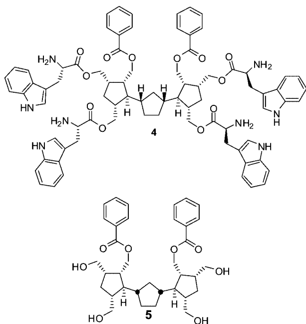
Figure 2. Structure of the lipid A binding tetra-tryptophan ter -cyclopentane derivative 4 , and the tetra-alcohol ter -cyclopentane synthetic precursor, 5 .
